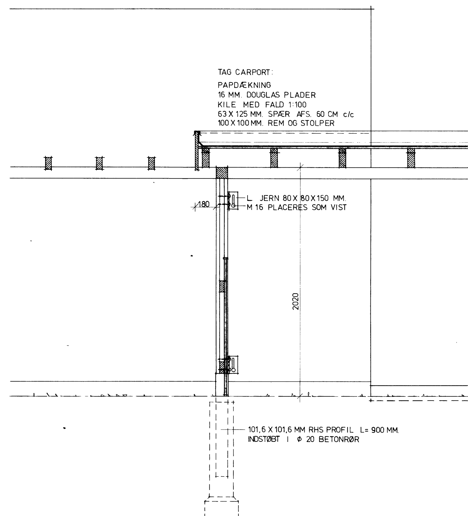
SNIT C - C
